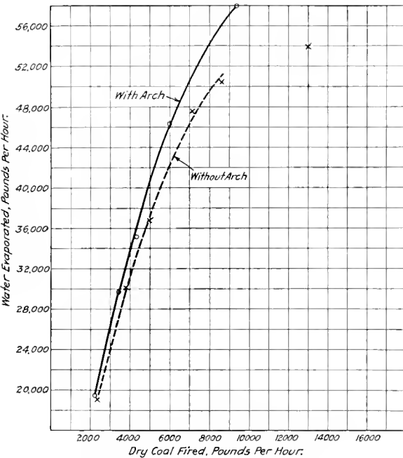
Fig. 1—Coal Fired and Water Evaporated
